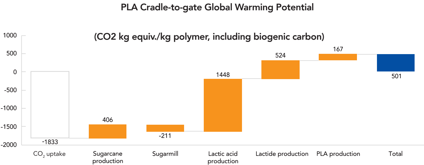
Figure [7]: LCA of PLA, Journal of Polymers and the Environment, (2019) [20]
